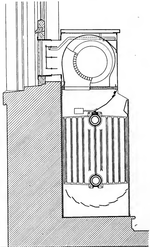
FIG. 12. TYPE OF UNIT HEATER SUITABLE FOR OFFICES, DRAFTING ROOMS AND SIMILAR OCCUPANCIES
